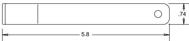
Scraper P/N 234350
